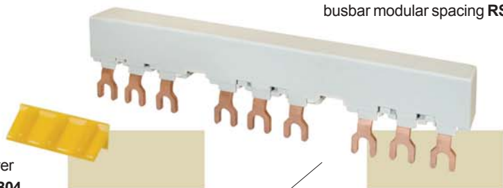
Insulated three-phase busbar modular spacing RSI-L
