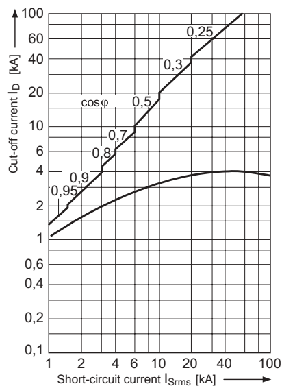
Current limiting characteristic for RMSI25-6
