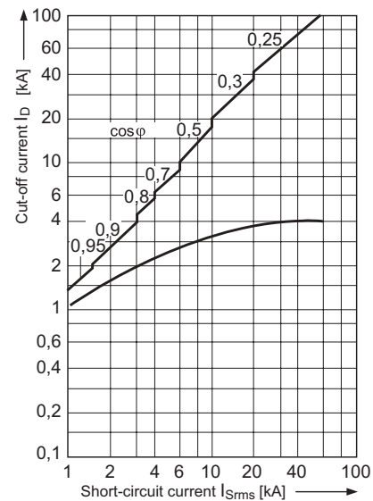
Current limiting characteristic for RMSI63-25
